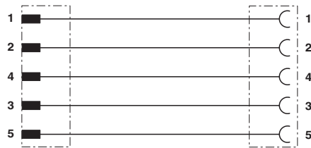
Circuit diagram
